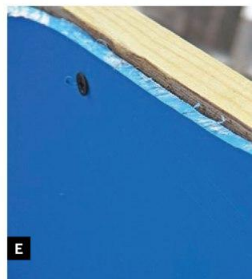
to be the top of the barrel. Figs. D–E: Build a frame of 1x2 lumber to fit exactly around the rim of your barrel, then screw the barrel to the frame.
