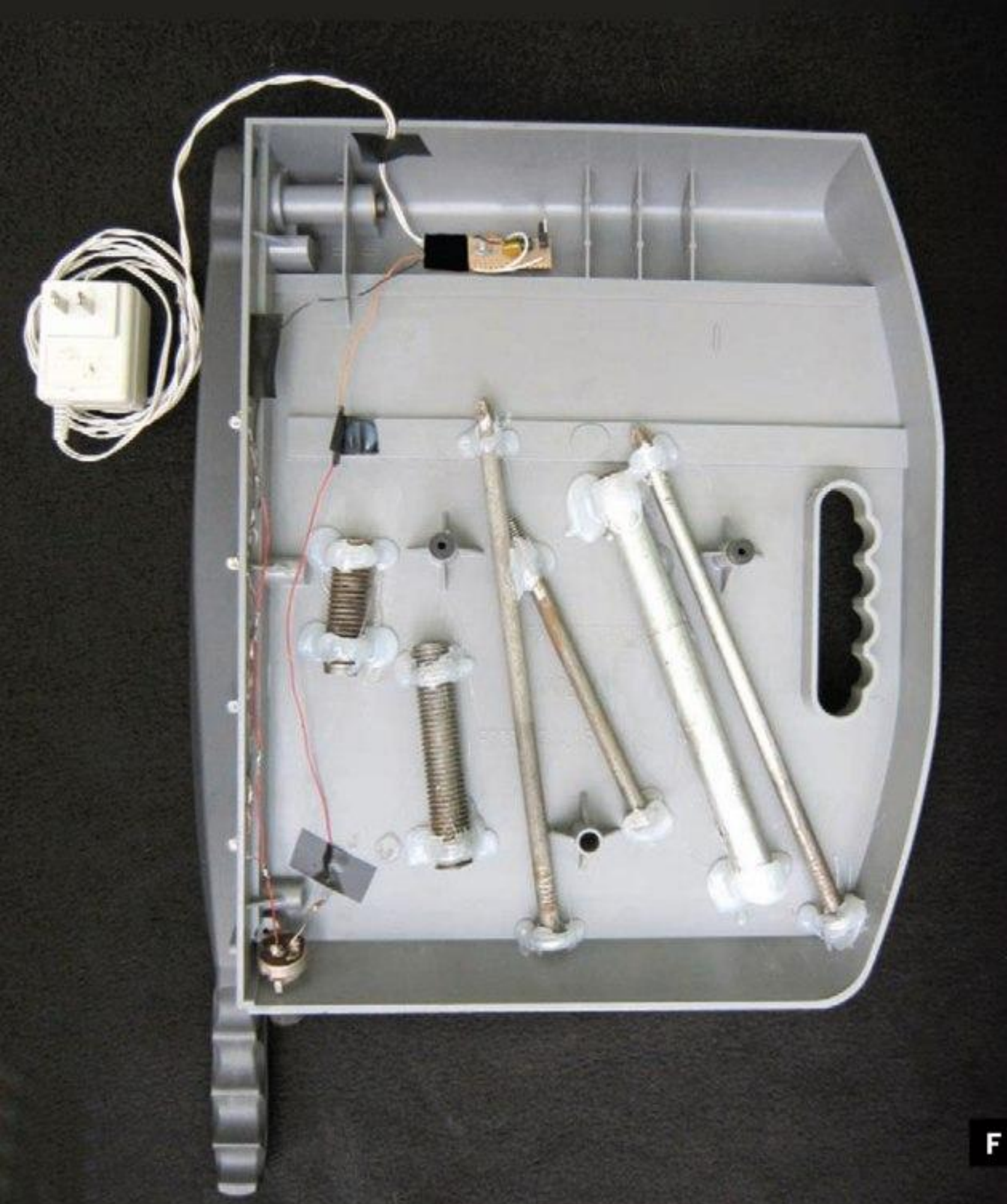
Fig. F: Add copious amounts of hot glue over both ends of all rods and heavy bolts to strap them in. Fig. G: You can add a ½"-wide scale in the recess in the top of the 02623X if you like.
